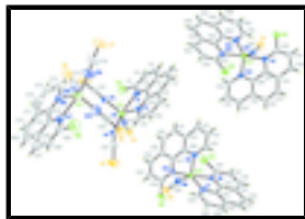
Fig. 1. The content of asymmetric unit of (I) showing the atomic numbering and 30% probability displacement ellipsoids.
